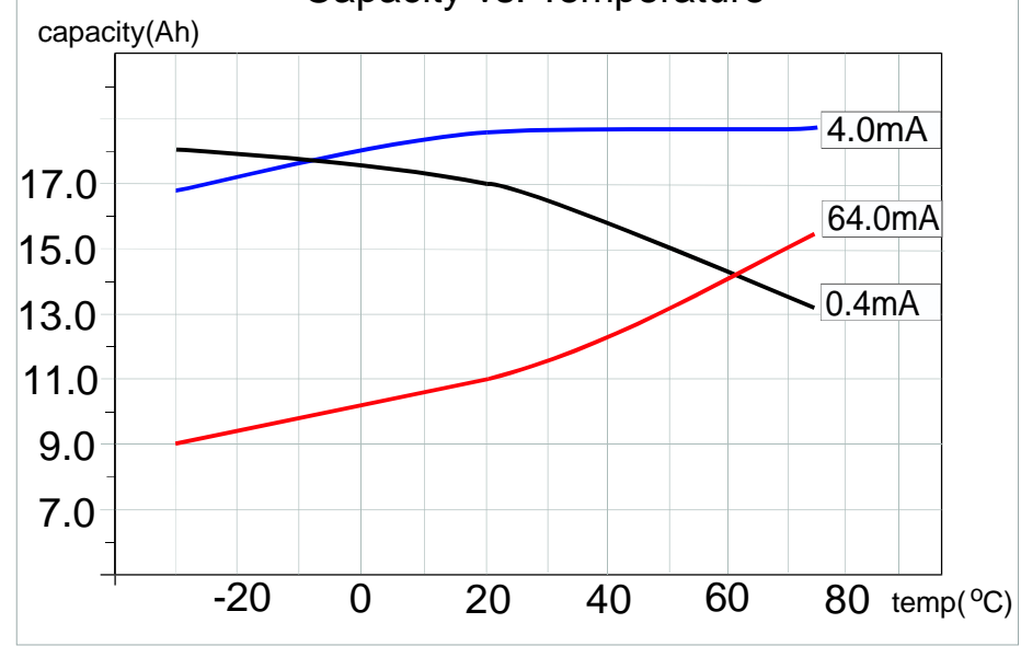
Capacity vs. Temperature
